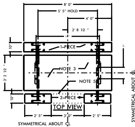
1 CONCRETE PAD PLAN 1/2" = 1' 0"
