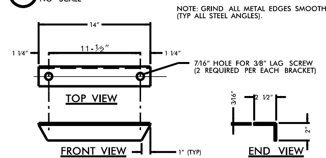
4 SEAT BRACKET - 8 REQ. NO SCALE
