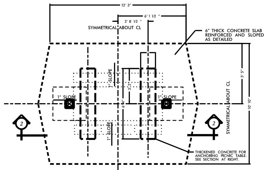
1 CONCRETE PAD PLAN 1/2" = 1' 0"
