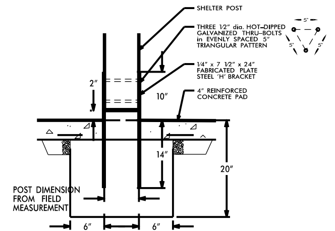
5 'H' BRACKET POST ANCHOR for RELOCATED PICNIC SHELTER N.T.S. 2 Required
