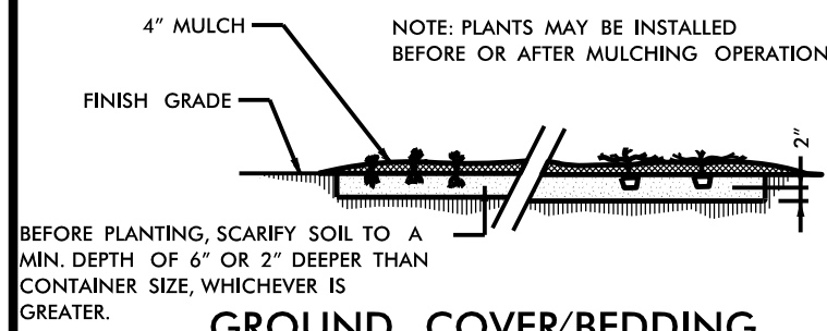
GROUND COVER/BEDDING PLANT DETAIL
