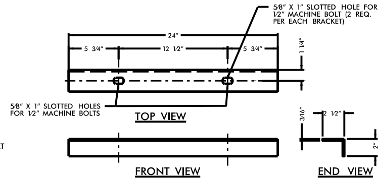
3 TABLETOP BRACKET - 2 REQ. NO SCALE
